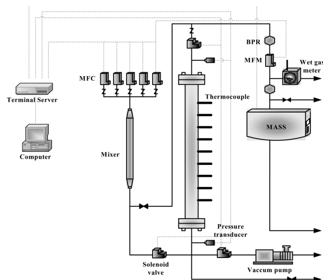
Fig. 1. Schematic diagram of breakthrough experiment apparatus.
