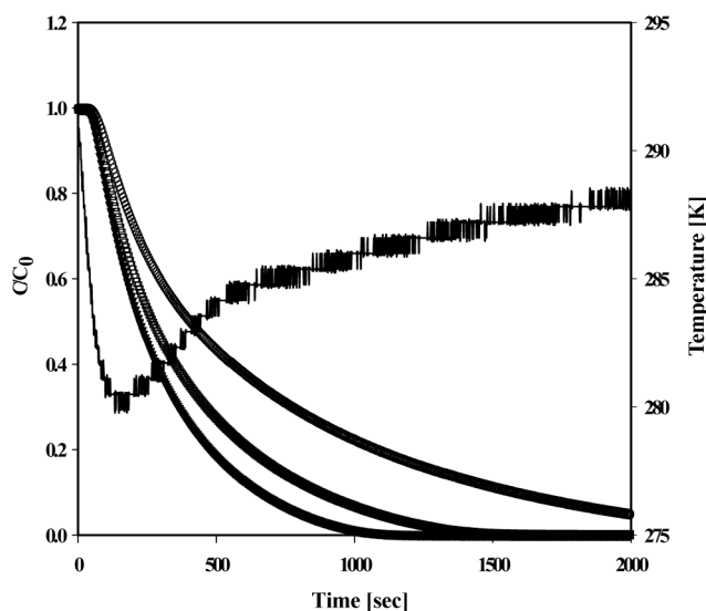
Fig. 6. Purge rate effect on H_2/CH_4 system at 1.2 atm blowdown pressure: \circ , CH_4 conc. at 1.5 LPM; \square , CH_4 conc. at 2.5 LPM; \nabla , CH_4 conc. at 3.5 LPM; —, temperature variation at CH_4 conc. at 1.5 LPM.
